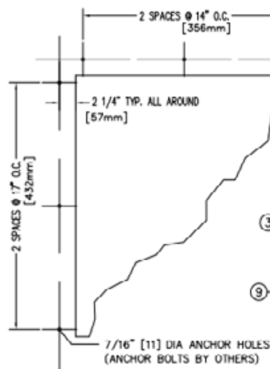
ANCHOR HOLE LAYOUT
